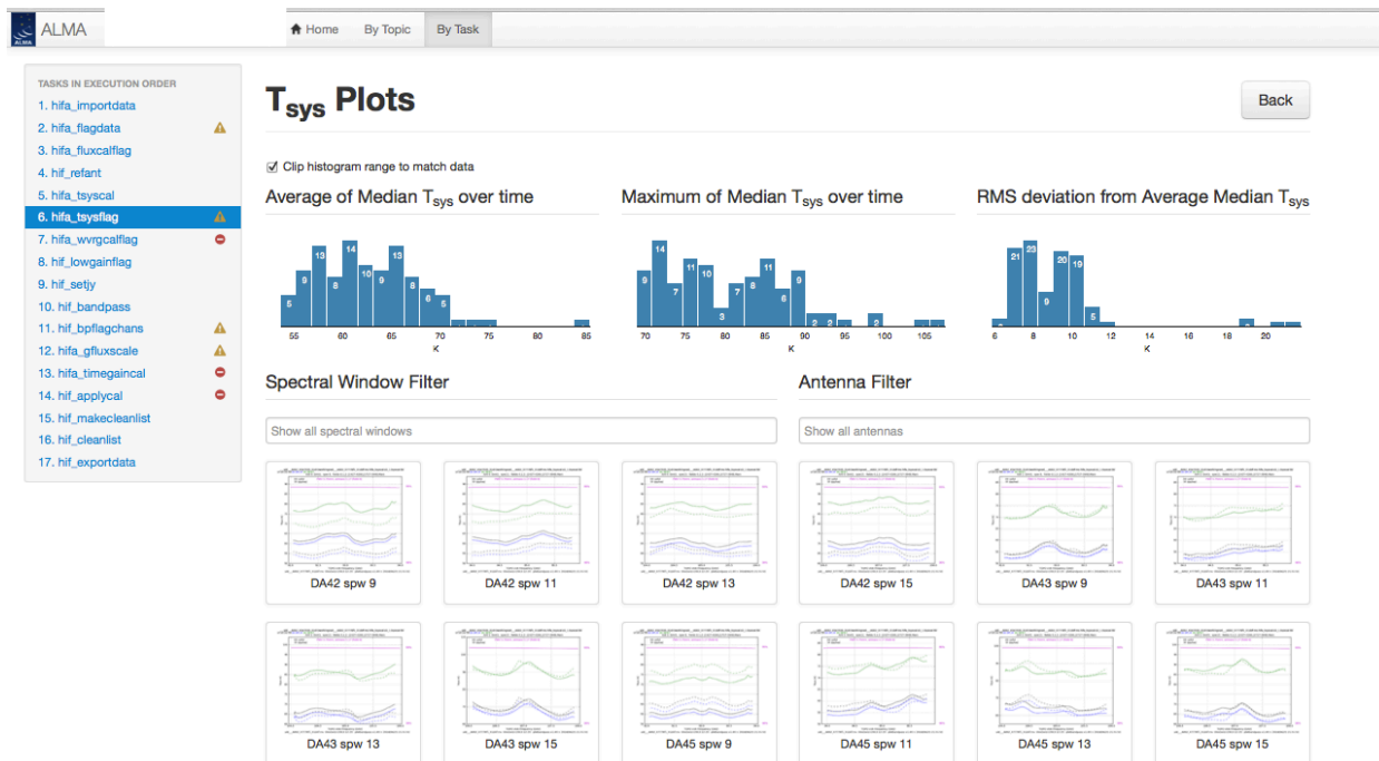
Figure 5: The Tsys plots for all antennas. Above the plots are histograms indicating the distributions of metrics based on the median Tsys.
