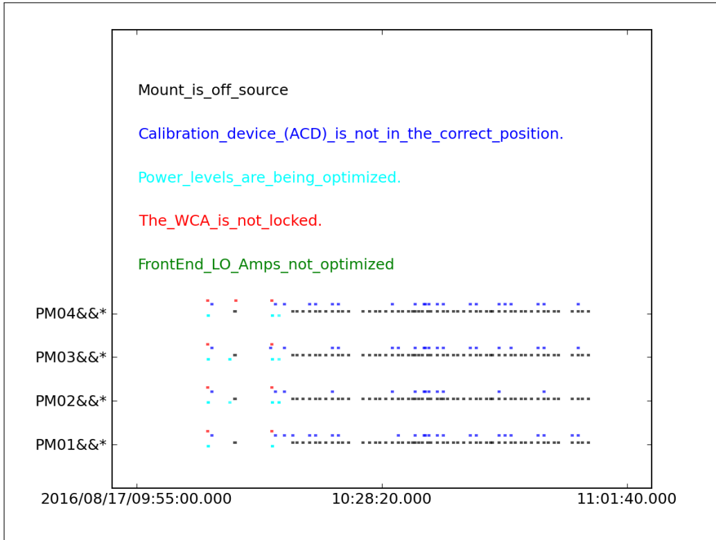
Figure 5.12: An example of a SD flagcmd plot from SB Target_a_1_08_TP (2015.1.00393.S) showing the a priori flagging.
