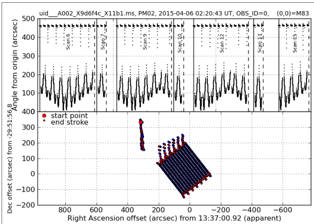
Figure 5.13: An example of a SD sampling plot from SB M83_b_03_TP (2013.1.01312.S) showing the observed footprints on the sky including the off-target positions used for measuring the sky signal for calibration.
