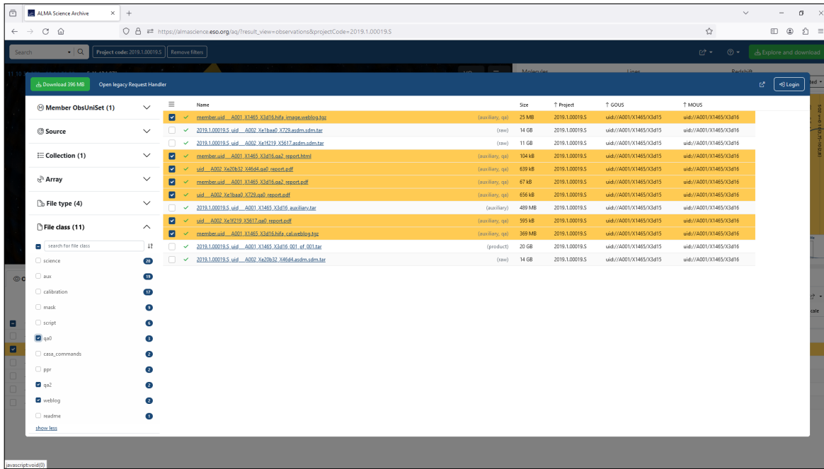
Figure 3.4: An example of how to use the Request Handler to select just the quality assurance data for download (based on the files from SB NGC4414_a_06_TM2 within project 2019.1.00019.S).
