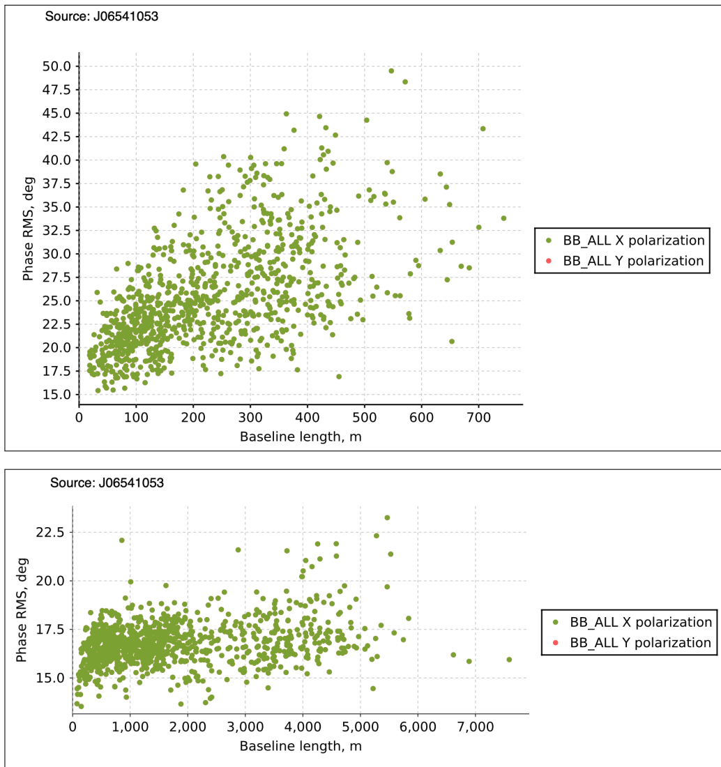
Figure 5.5: Examples of the phase RMS behaviour for various baseline lengths, with Band 6 data for calibrator J0654-1053 from SB Z_CMa_a_06_TM2 (2018.1.01131.S) in the top panel and from SB Z_CMa_a_06_TM1 (2016.1.00110.S) in the bottom panel.
