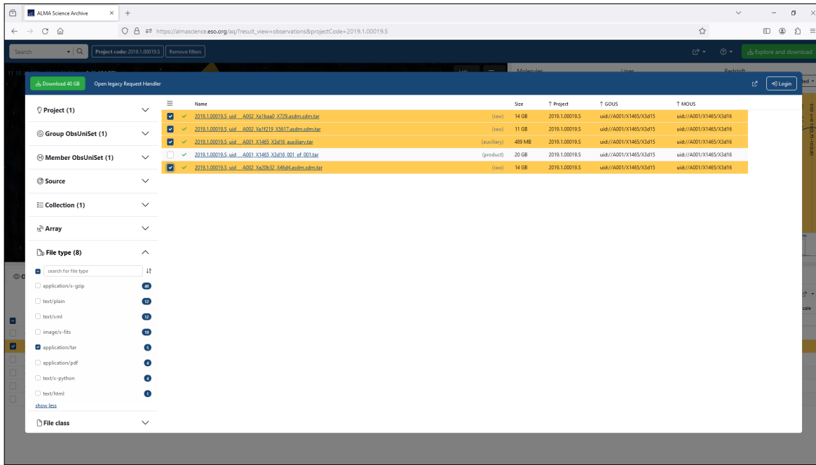
Figure 3.5: An example of how to use the Request Handler to select the raw and auxiliary files for download (so as to create new images). This is example is based on the files from SB NGC4414_a_06_TM2 within project 2019.1.00019.S.
