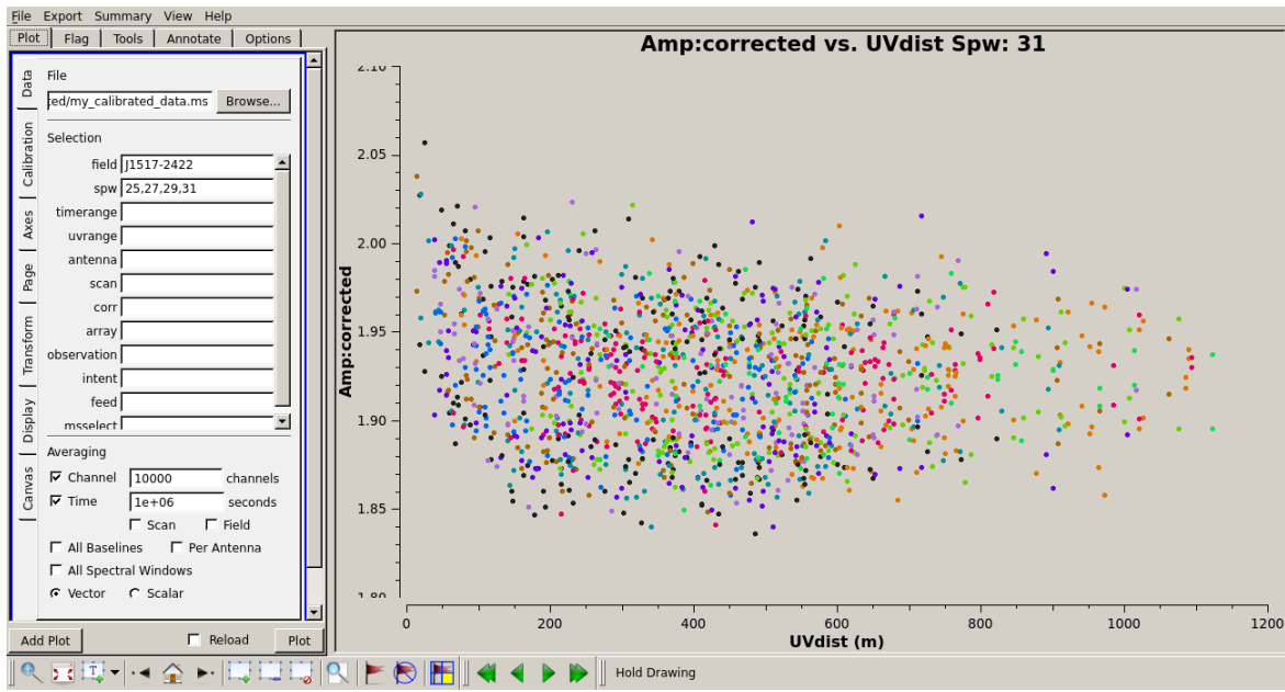
Figure 5.21: An example of the plotms GUI showing amplitude versus uv -distance within spectral window 31 for the bandpass calibrator J1517-2422.
