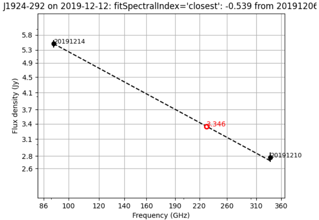
Figure 11.2: Flux density vs. frequency plot of J1924-292 generated by the getALMAFlux task given in the example above.
