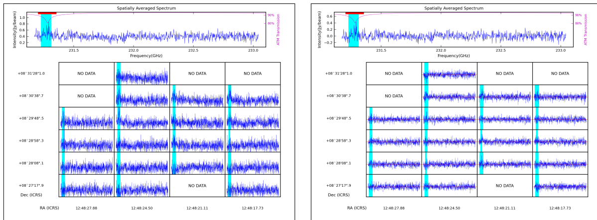
Figure 5.20: Examples of the hsd_baseline plots for SB NGC_4698_a_06_TP (2019.1.00763.L) showing spectral window 19 before (left panel) and after (right panel) the baseline subtraction.
