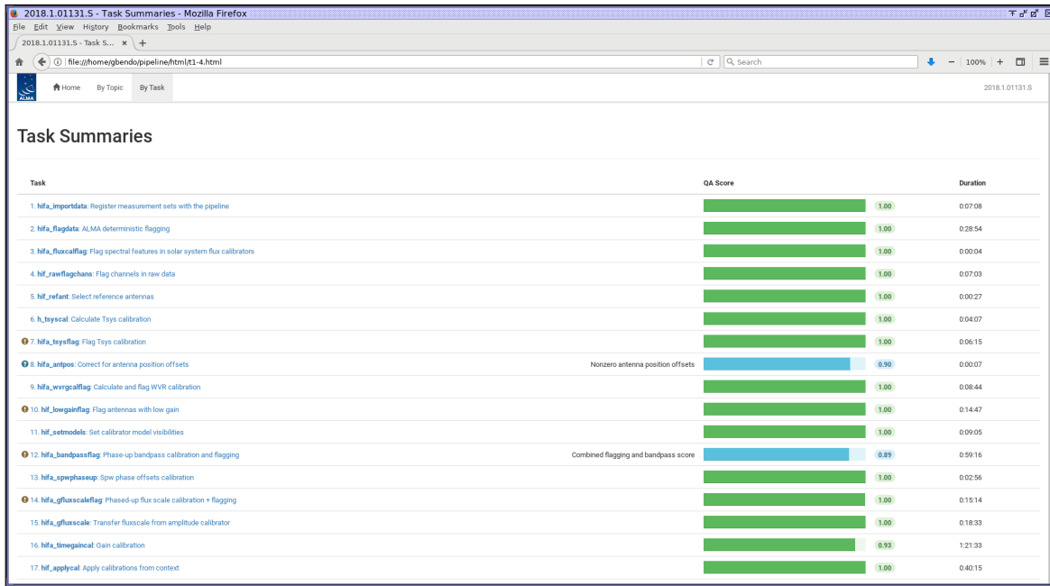
Figure 5.17: An example of a WebLog “By Task” page for SB Z_CMa_a_06_TM1 (2018.1.01131.S).
