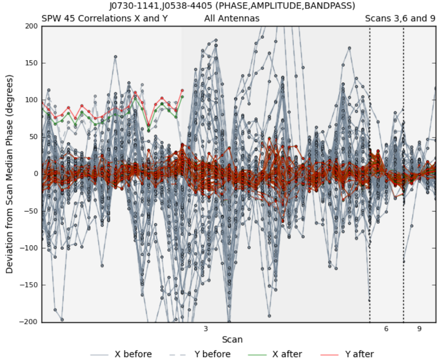
Figure 5.19: An example of the plot from the WebLog task hifa_wvrgcalflag showing the deviation from median phases versus time for the calibrator targets in SB Z_CMa_a_06_TM1 (2018.1.01131.S).
