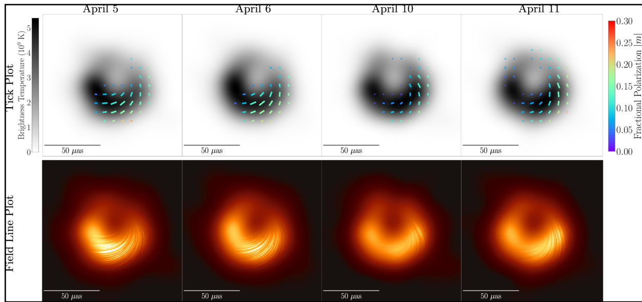
Figure 10: Images of the event horizon of the supermassive black hole at the centre of M87, obtained by the Event Horizon Telescope over four days in April 2017. Two visualization schemes are used to show the polarization orientation and intensity, which are related to the magnetic field in the region. In the top row, total intensity, polarization fraction, and EVPA are plotted. In the bottom row, the polarization “field lines” are plotted atop an underlying total intensity image. (Credits: EHT Collaboration, 2021, ApJL , 9310, L12)
