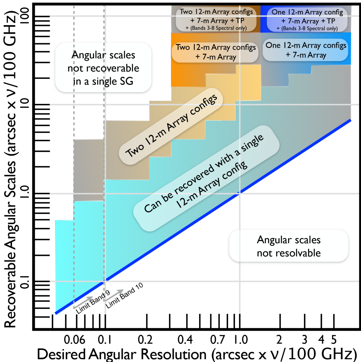
Figure 28: This figure links Desired Angular Resolution to the Maximum Recoverable Scale (MRS) in Cycle. The desired angular resolution determines the largest baselines (and hence the configuration) of the 12-m Array. The observations from that configuration can recover structure over a range of angular scales; for example, an observation at 1" resolution at 100 GHz can recover structure over size-scales from ~1" to ~11" (cyan region). Structures larger than the "Maximum Recoverable Scale" (MRS; see p. 24) are "resolved out" by the interferometer. Structure larger than the MRS may be recovered either by adding observations using a smaller 12-m Array configuration, by adding observations using the 7-m Array, or by adding both another configuration and the 7-m Array. Still larger scale structure may be recovered for Bands 3-8 spectral observations by adding data from the Total Power (TP) array. To use this figure, you first need to scale your desired angular resolution and LAS by the factor (\nu/100\text{GHz}) , where \nu is your desired frequency in GHz. For example, suppose you wanted to observe at 300 GHz (Band 7) with angular resolution 0.4" and LAS of 10". These become 1.2" and 30" respectively when scaled to 100 GHz. Reading from the figure above, two 12-m Array configurations plus the ACA 7-m Array would be needed to recover all angular scales. (The OT will automatically determine the required combination of arrays/configurations to achieve the resolution/LAS you require.) Note that adding configurations or the ACA will significantly increase the required observing time. See Chapter 7 of the Technical Handbook and the Proposer's Guide in the Call for Proposals for details and restrictions. Note that angular resolutions finer than (0.057" \times 100 \text{ GHz}/\nu) are not permitted for Band 9, and angular resolutions finer than (0.096" \times 100 \text{ GHz}/\nu) are not permitted for Band 10 ("Limit Band 9" and "Limit Band 10" on figure above).
